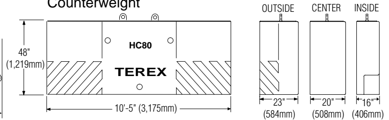
Counterweight
