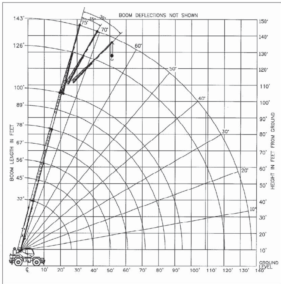
Range Diagram (32' - 100' boom)
